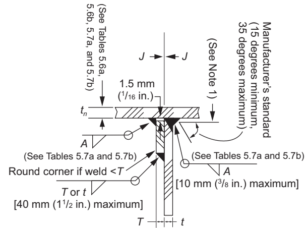
Nozzle
